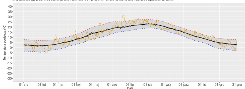
HEL - variability of the maximum daily air temperature (TMAX) in 2021 with reference to long-term characteristics 1991-2010; maximum daily air temperature in 2021 (orange line), long-term average (black line), quantiles: 95% (red line) and 5% (blue line) - smoothed with locally weighted polynomial regression
