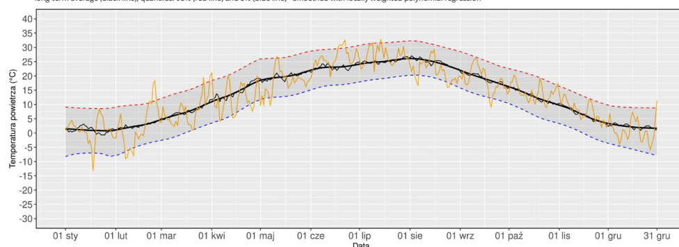
WARSAW-OKĘCIE - variability of the maximum daily air temperature (TMAX) in 2021 with reference to long-term characteristics 1991-2010; maximum daily air temperature in 2021 (orange line), long-term average (black line), quantiles: 95% (red line) and 5% (blue line) - smoothed with locally weighted polynomial regression
