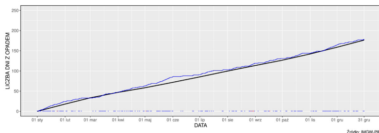
Cumulative number of days with precipitation (daily precipitation total \geq 0.1 mm) in 2021 – blue line with reference to the cumulative mean monthly number of days with precipitation in the long-term period 1991-2020 – bold black line, blue points – days with precipitation, red points – days with precipitation >10 mm, Lublin – Radawiec
