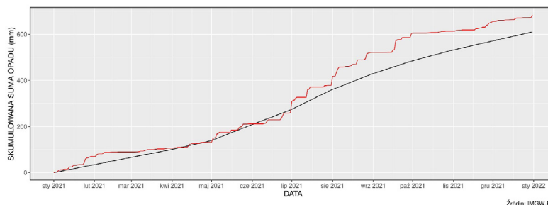
Cumulative daily precipitation totals in 2021 – red line with reference to cumulative long-term normals 1991-2020 – black line, Chojnice
