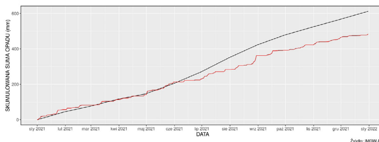
Cumulative daily precipitation totals in 2021 – red line with reference to cumulative long-term normals 1991-2020 – black line, Lublin-Radawiec
