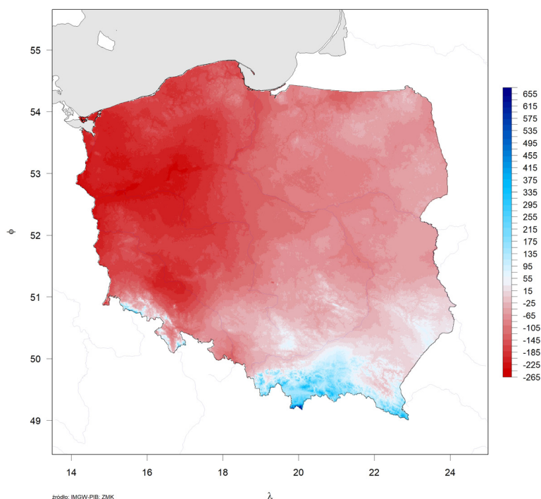
Total Climatic Water Balance - May - October 2021
