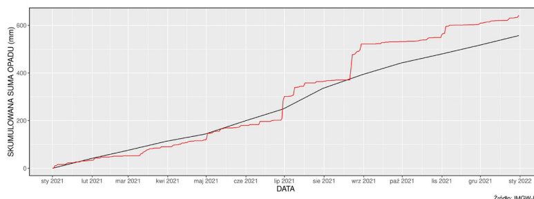
Cumulative daily precipitation totals in 2021 – red line with reference to cumulative long-term normals 1991-2020 – black line, Stubice
