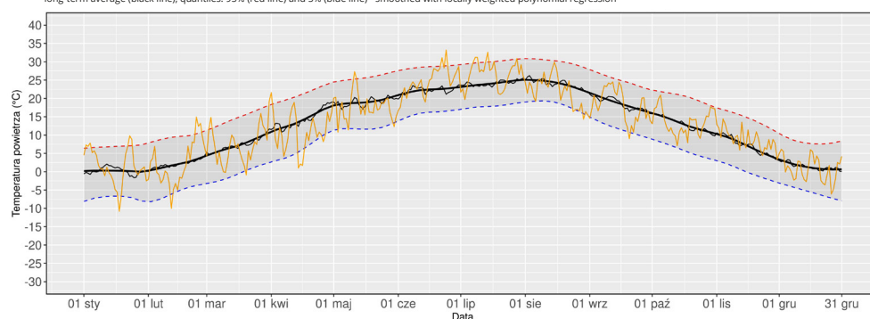
KROSNO - variability of the maximum daily air temperature (TMAX) in 2021 with reference to long-term characteristics 1991-2010; maximum daily air temperature in 2021 (orange line), long-term average (black line), quantiles: 95% (red line) and 5% (blue line) - smoothed with locally weighted polynomial regression
