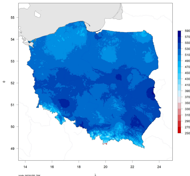
Total Evapotranspiration - May - October 2021
